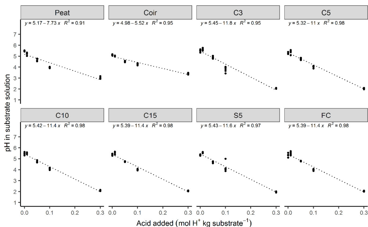
Figure 7. Linear regression for the determination of pH buffering capacity of peat, coir, and six processed miscanthus substrates. Each point represents for one sample. For each substrate at each proton concentration, there are 5 replicates. Miscanthus × giganteus was harvested with a forage harvester (FC, field-chips), then processed with a mechanical fraying facility through a 5-mm screen (S5, shreds) or a hammermill with screen sizes of 15, 10, 5, and 3 mm (C15, C10, C5, and C3, chips).
