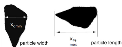
Figure 1. Two main particle size parameters analyzed with Particle Analyzer Camsizer: particle width ( x_{\text{cmin}} , the shortest chord diameter), particle length ( x_{\text{Femax}} , the longest Feret diameter) (adapted from [44].).
