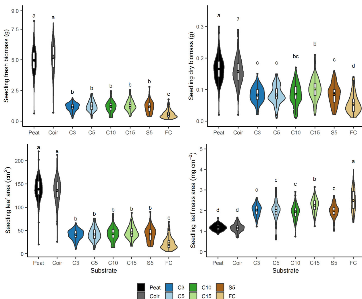
Figure 10. Seedling growth on peat, coir, and six processed miscanthus substrates: seedling fresh biomass, dry biomass, leaf area and leaf mass area. The violin plot represents the data distribution of 72 single seedlings at each substrate (4 replicates × 18 seedlings). The boxplot inside represents median, interquartile ranges and mean value as point. The width of the violin represents the number of value in each range. Different small letters indicate statistically significant differences in means among substrates (Tukey's HSD, p \leq 0.05 , mean \pm standard deviation, n = 72 ). Miscanthus × giganteus was harvested with a forage harvester (FC, field-chips), then processed with a mechanical fraying facility through a 5-mm screen (S5, shreds) or a hammermill with screen sizes of 15, 10, 5, and 3 mm (C15, C10, C5, and C3, chips).
