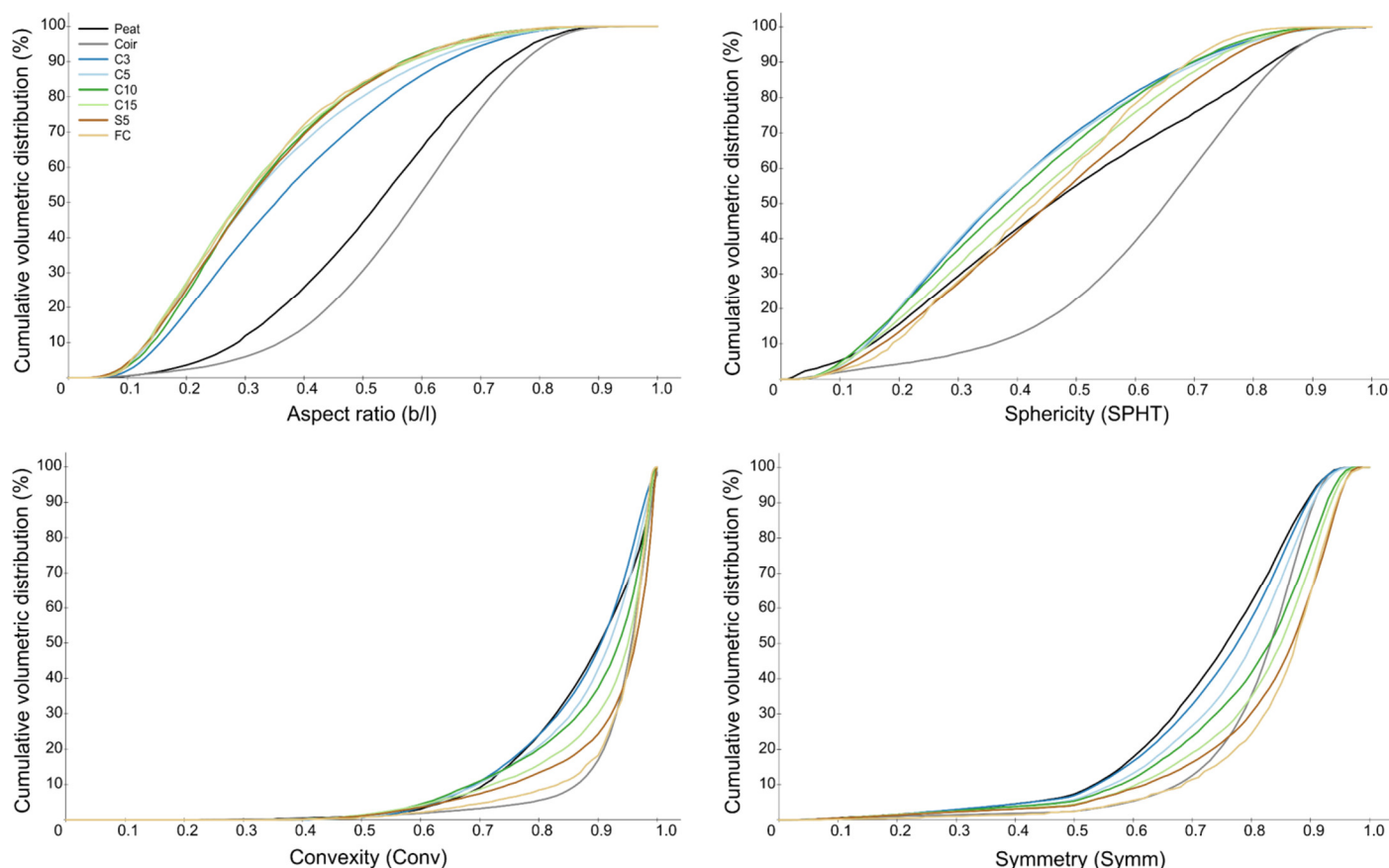
Figure 3. Volumetric distribution of particle shape of peat, coir, and processed miscanthus substrates analyzed with dynamic image analysis. The curve represents for one measurement of each substrate. Miscanthus \times giganteus was harvested with a forage harvester (FC, field-chips), then processed with a mechanical fraying facility through a 5-mm screen (S5, shreds) or a hammermill with screen sizes of 15, 10, 5, and 3 mm (C15, C10, C5, and C3, chips).
