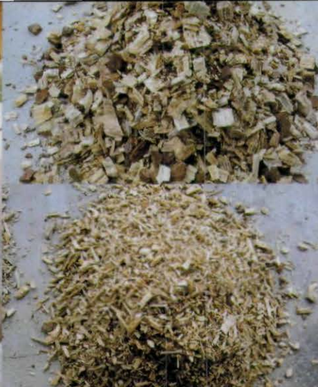
A hammer mill can be fitted with different-sized screens to grind coarse wood chips into any particle size to produce a substrate with physical characteristics similar to pine bark or peat-based mixes.
